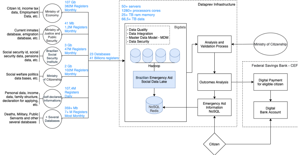
Figure 1 – Conceptual Model of Dataprev’s Emergency Aid solution.
