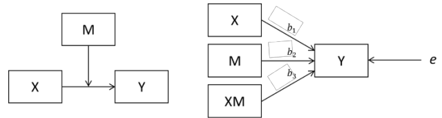
Fig. 1 Conceptual and statistical diagrams of the simple moderation model
