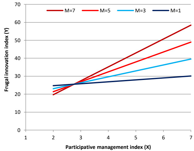
Graph 3 Graph showing the dispersion of the relationship between X (participative management index) and Y (frugal innovation index), for various value of the variable M (decentralization level)
